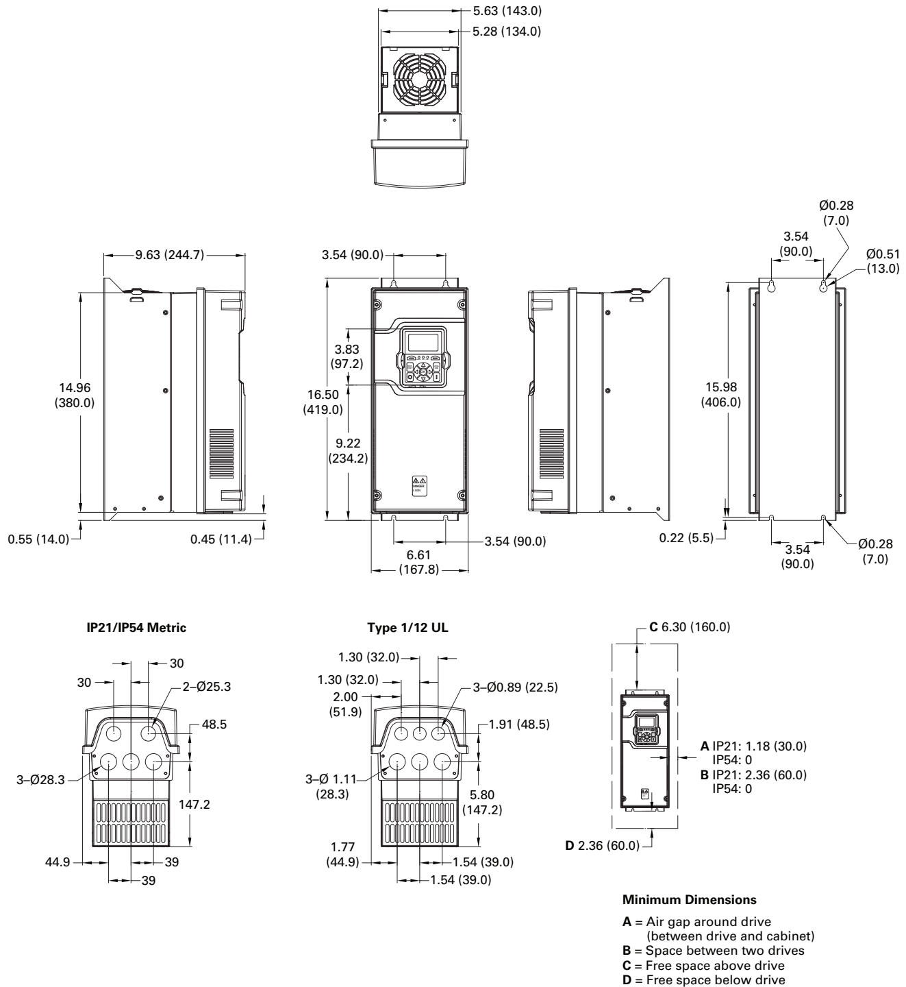
Figure 43. FR2 dimension drawing
