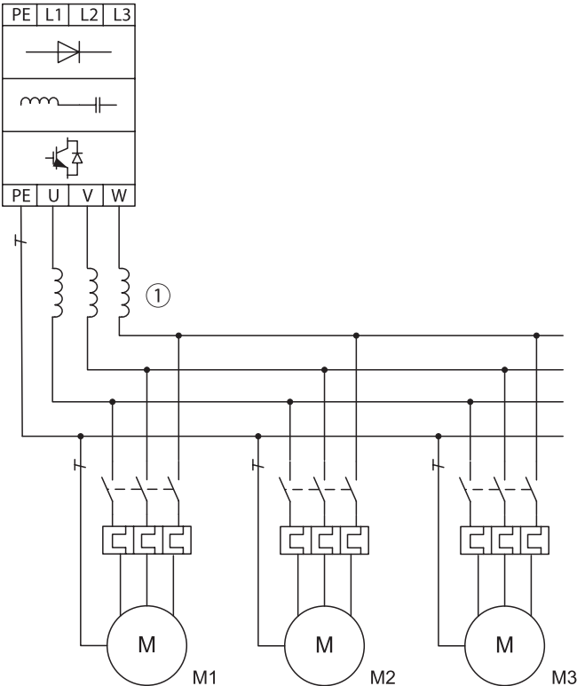
Figure 14. Parallel connection
