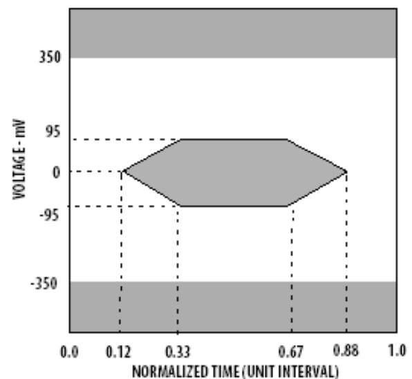
Figure 3b. Transmitter Differential Input Compliance Mask at B
