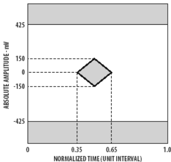
Figure 3a. Receiver Electrical Optical Eye Mask Definition
