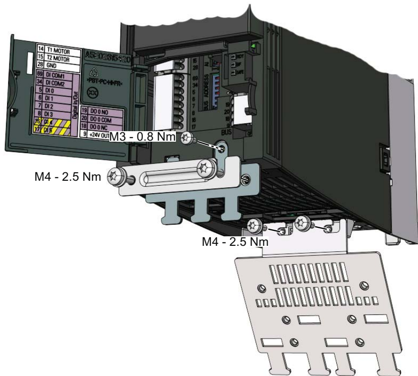
Frame Size A & B
