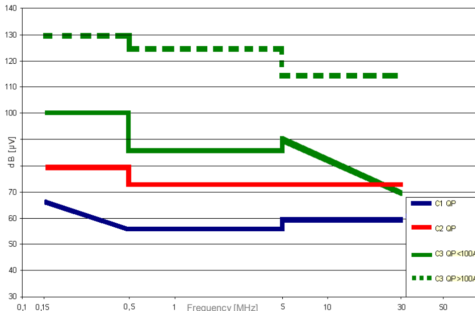
Permissible interference voltage limits in dB[ \mu V] for categories C1, C2 and C3 (QP = quasi-peak values)
