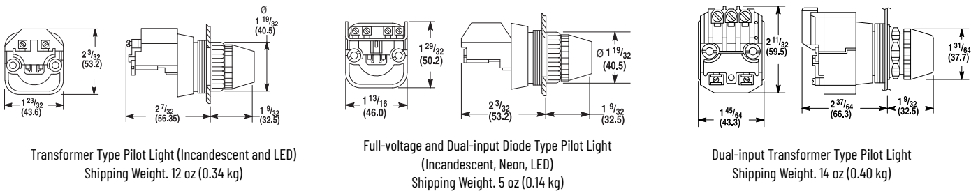
Figure 4 - Push-to-test Pilot Lights – Illuminated Push Buttons, Illuminated Push-pull and Twist, or Pull Release Push Buttons
