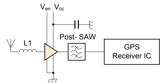
Application diagram for wearable health and fitness device, showing the input-match inductor (L1) and a post-SAW
