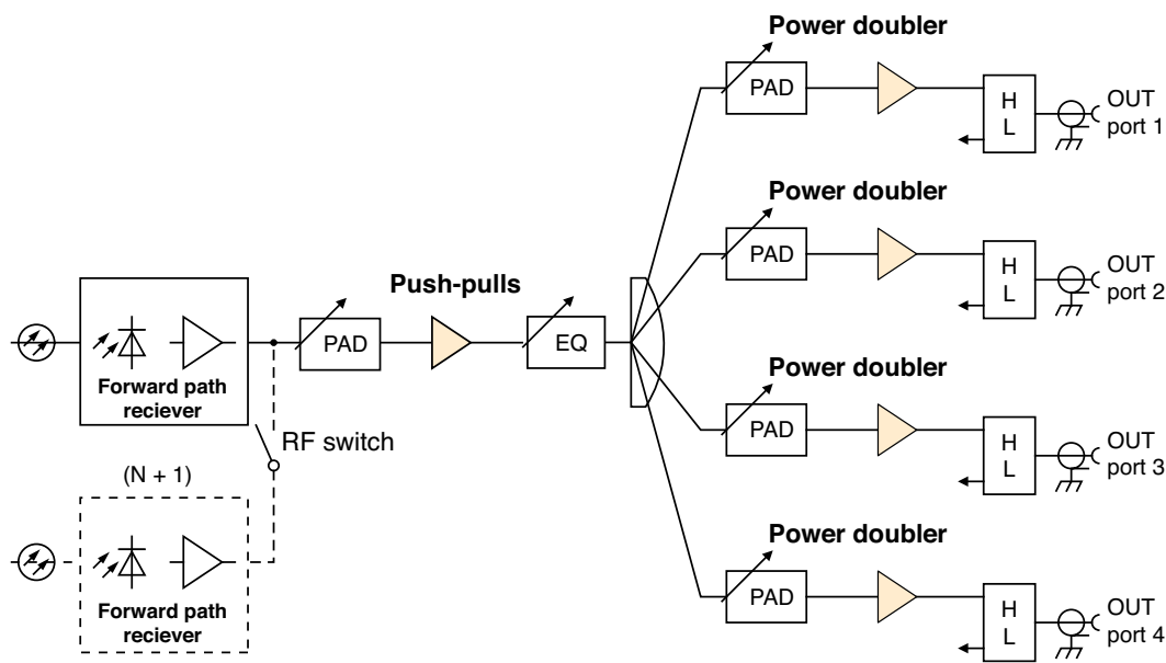
Application diagram of CATV optical node with multiple OUT ports for 1 GHz networks
