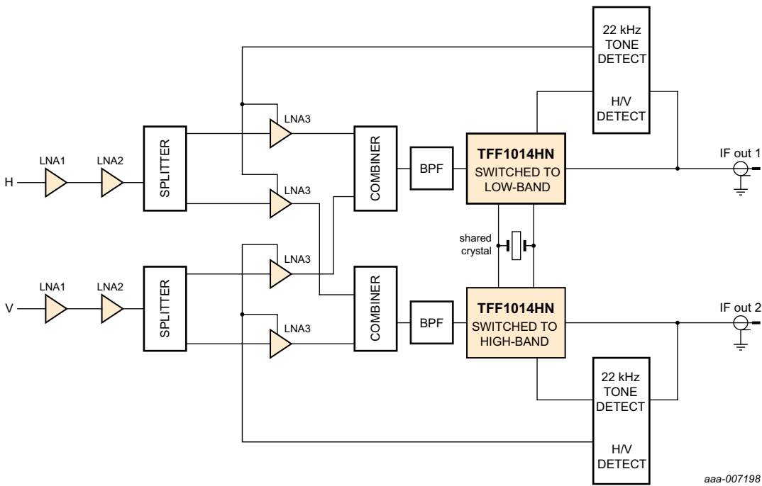
Application diagram of a twin LNB based on the TFF101x
