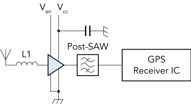
Application diagram of wearable health and fitness device, showing the input-match inductor (L1) and a post-SAW
