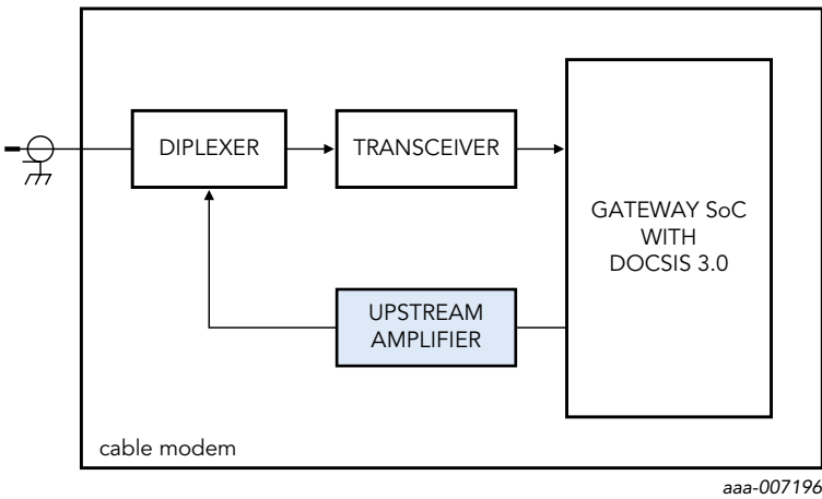
Application diagram of a DOCSIS cable modem with the BGA3031 upstream amplifier
