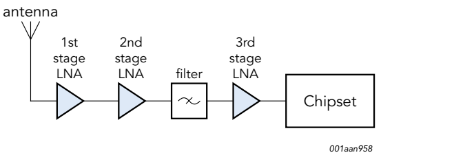
Application diagram of an SDARS Active Antenna LNA - 2320-2332.5 (SIRIUS, 3 stages)
