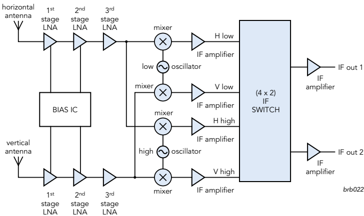
Application diagram of a twin LNB with discrete components
