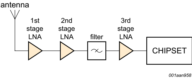
Application diagram of an SDARS Active Antenna LNA - 2320-2332.5 (SIRIUS, 3 Stages)
